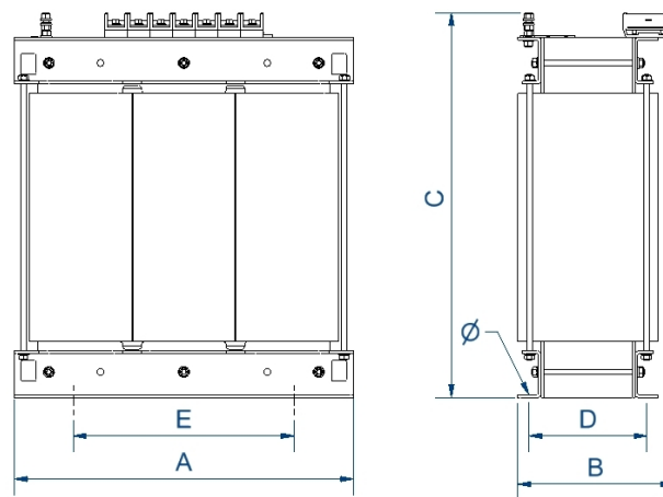
Dimensions (AxBxCxDxE): 1083x700x1220x600x690 mm 18Ø
