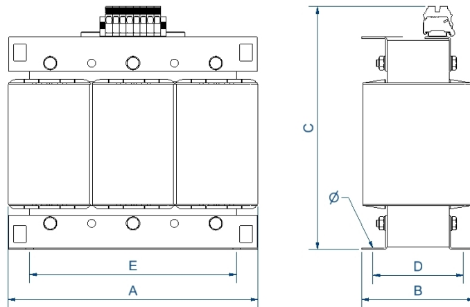
Dimensions (AxBxCxDxE): 360x164x371x142x300 mm 11Ø
