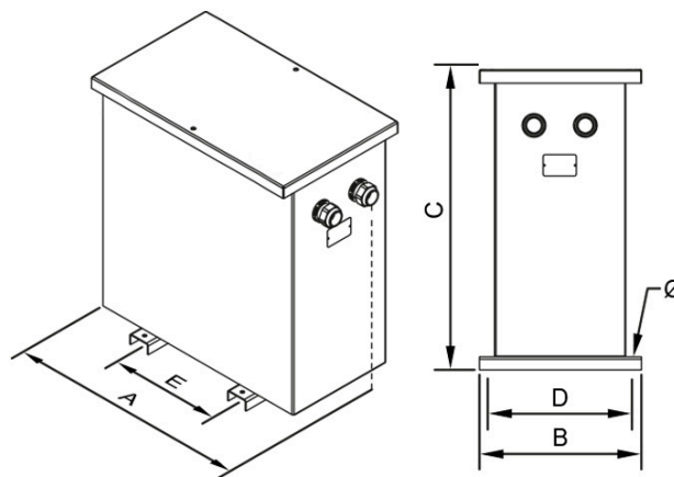
Dimensions (AxBxCxDxE): 1527x1000x1746x806x684 mm 18°
